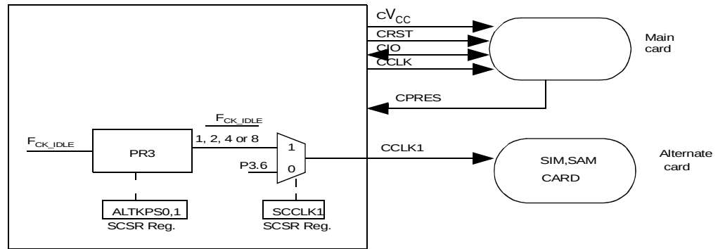
Figure 22. Alternate Card
